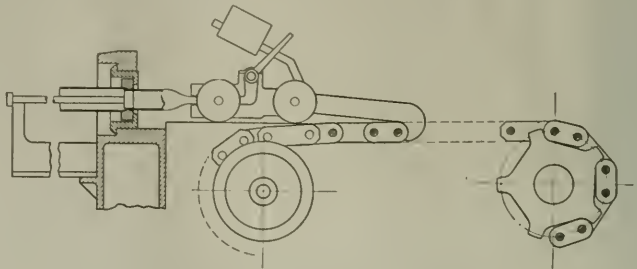
DIAGRAM OF COLD-DRAWING OPERATION
